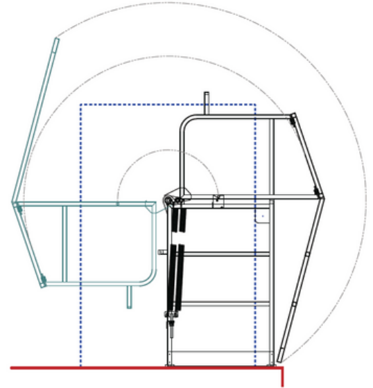
Single Pallet Gate Unit opening illustration with blue dotted load line
